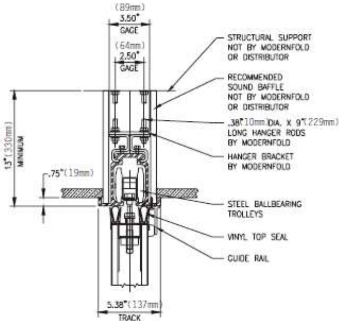
#30 Track system Standard Spacing
