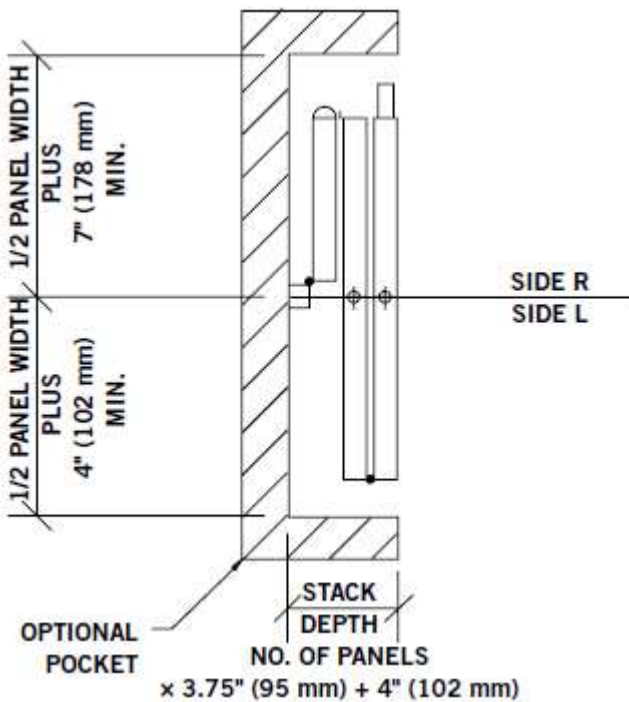
Single Hinged Panel Closure
