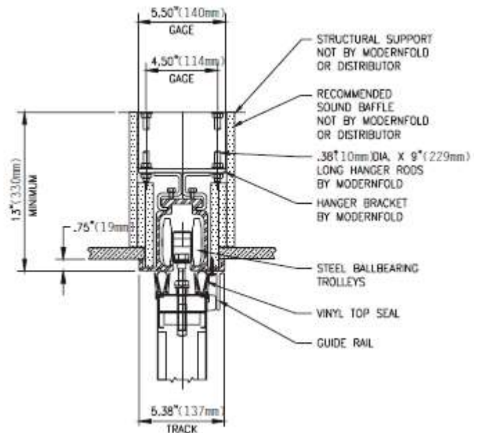
#30 Track System Optional Wider Spacing
