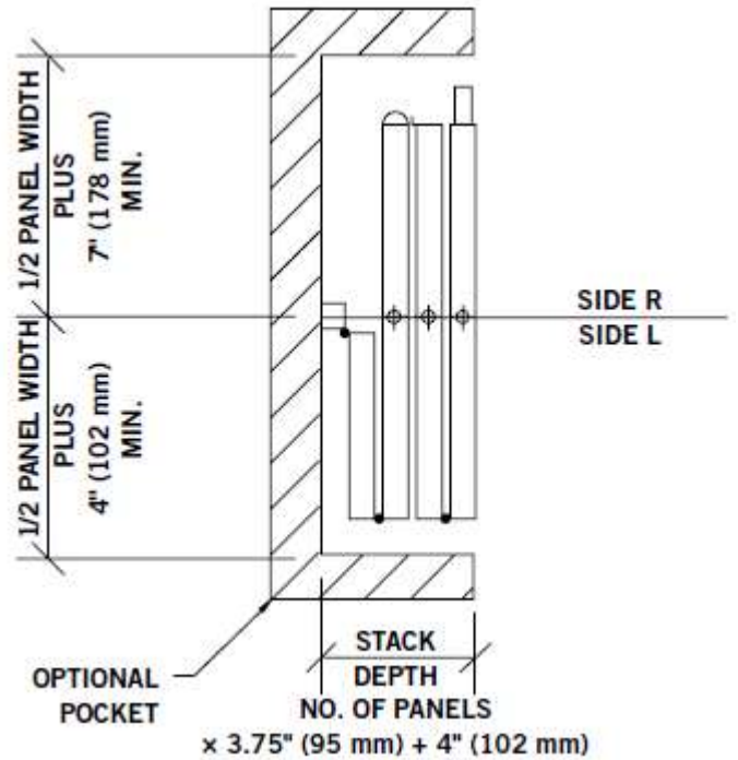
Bi-Fold Hinged Panel Closure
