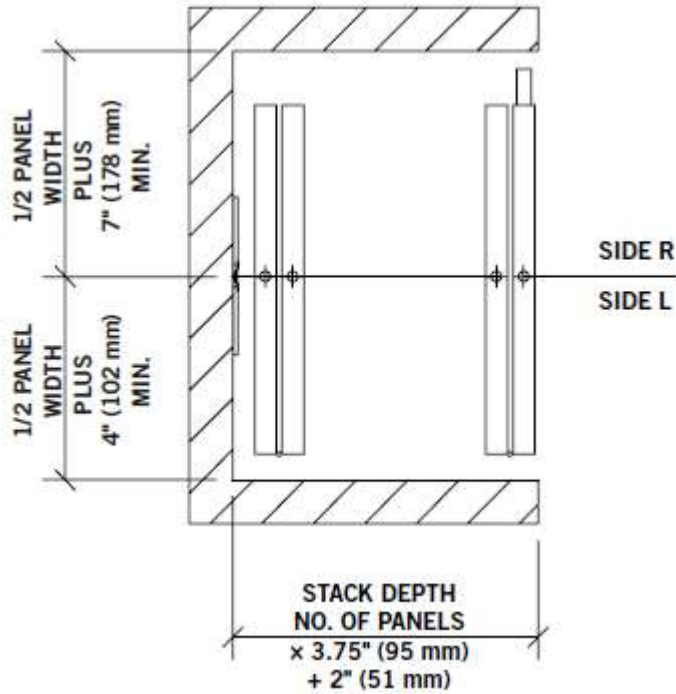
Single Hinged Panel Closure
